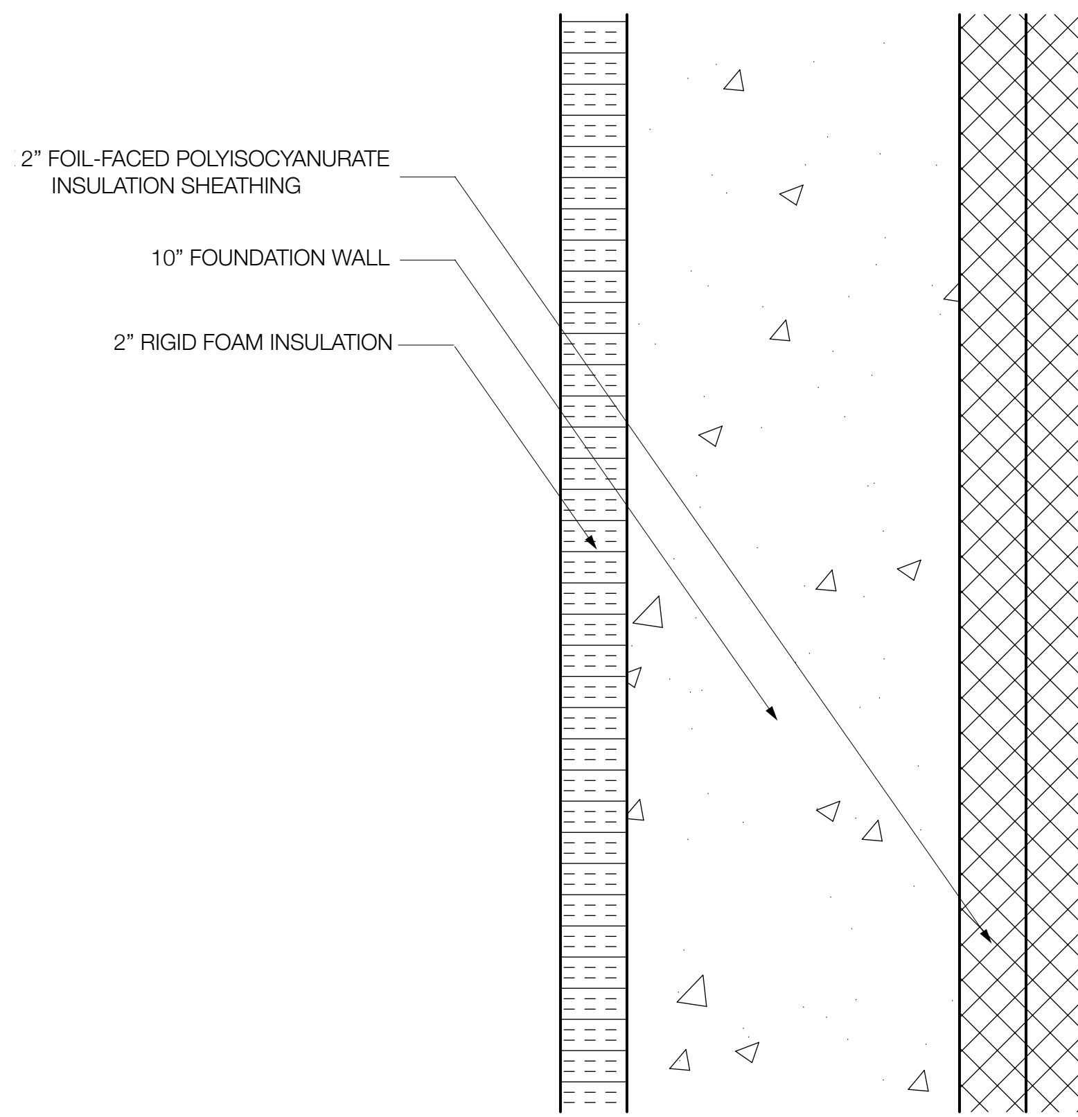
Basement Wall Section
